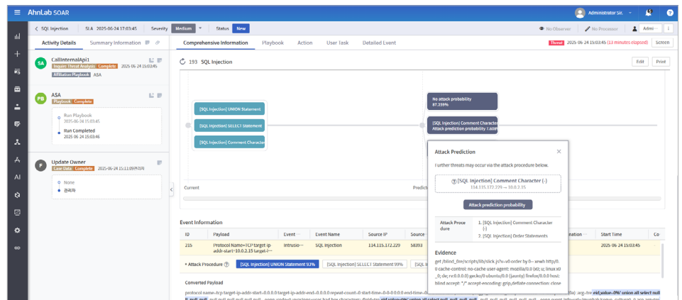
Figure 3. Proactive Response to Additional Attacks through AI-Based Correlation Analysis
